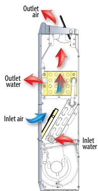
Heating Static convector mode Natural convection
