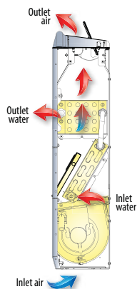
Heating Static convector mode Extra low speed
