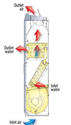
Heating Fan coil mode Low, medium and high speed
